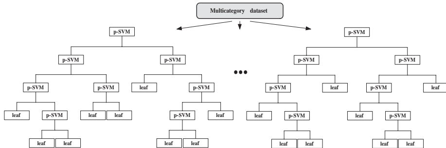
Fig. 1: Embedded proximal SVMs in an ensemble of decision trees for multi-category data classification
